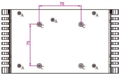
VESA 75 Mounting
